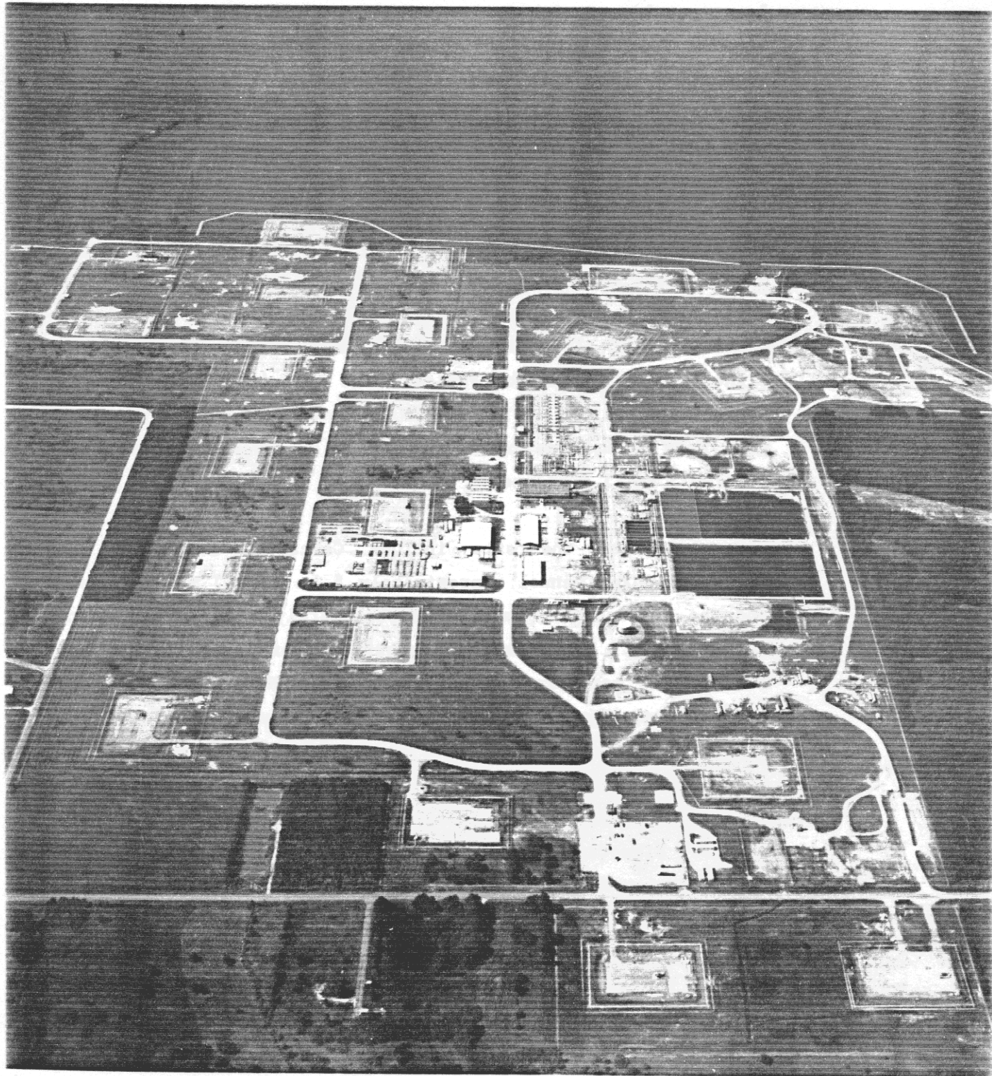
Figure 1-8. West Hackberry SPR Site
